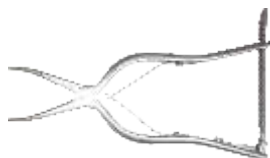
Compressing Forceps Part No. B 778001000
